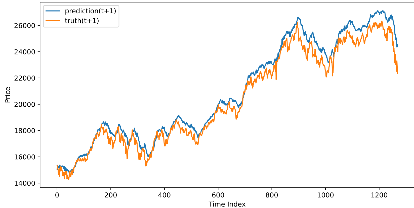
LDENet 1.5 - Prediction vs Truth
